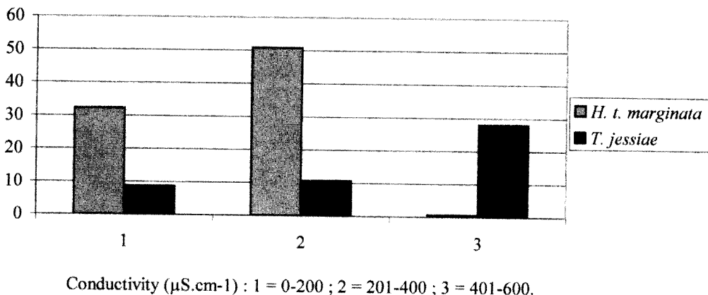
Fig. 46 : Average numbers of individuals of Leptophlebiidae collected per station, in function of conductivity.
