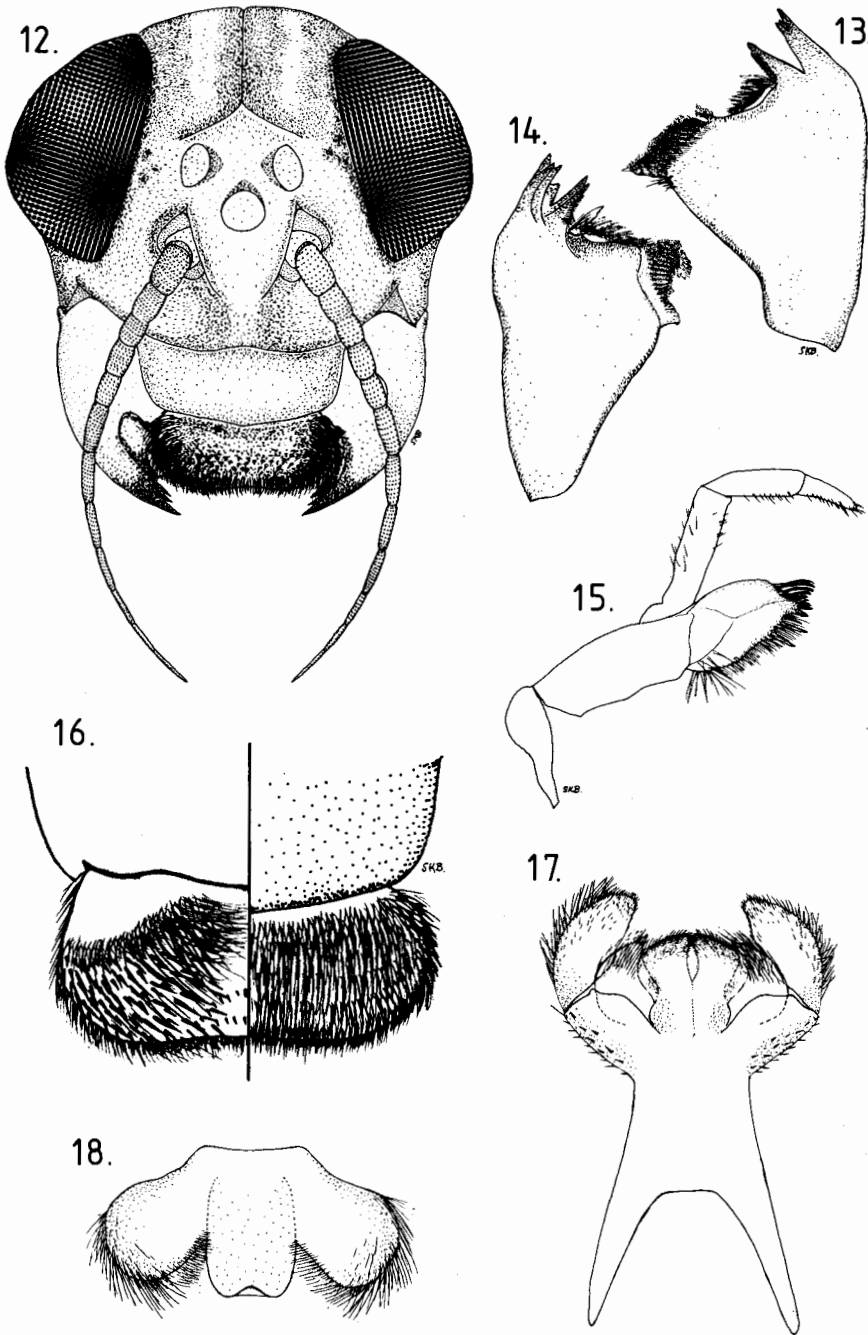
Figs. 12-18. Mature nymph of Siphonisca aerodromia : 12 - frontal view of head; 13 - right mandible; 14 - left mandible; 15 - maxillae with maxillary palp; 16 - labrum with dorsal view to right; 17 - labium with glossa and paraglossa; 18 - superlingua.
