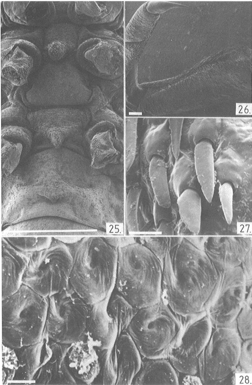
Figs. 25-28. Mature nymph and egg of Siphonisca aerodromia : 25 - ventral view of thoracic sterna and sternal setae, bar = 1000 \mu m; 26 - right prothoracic leg, bar = 100 \mu m; 27 - closeup of sternal setae, bar = 10 \mu m; 28 - photograph of surface structures of egg, bar = 10 \mu m.
