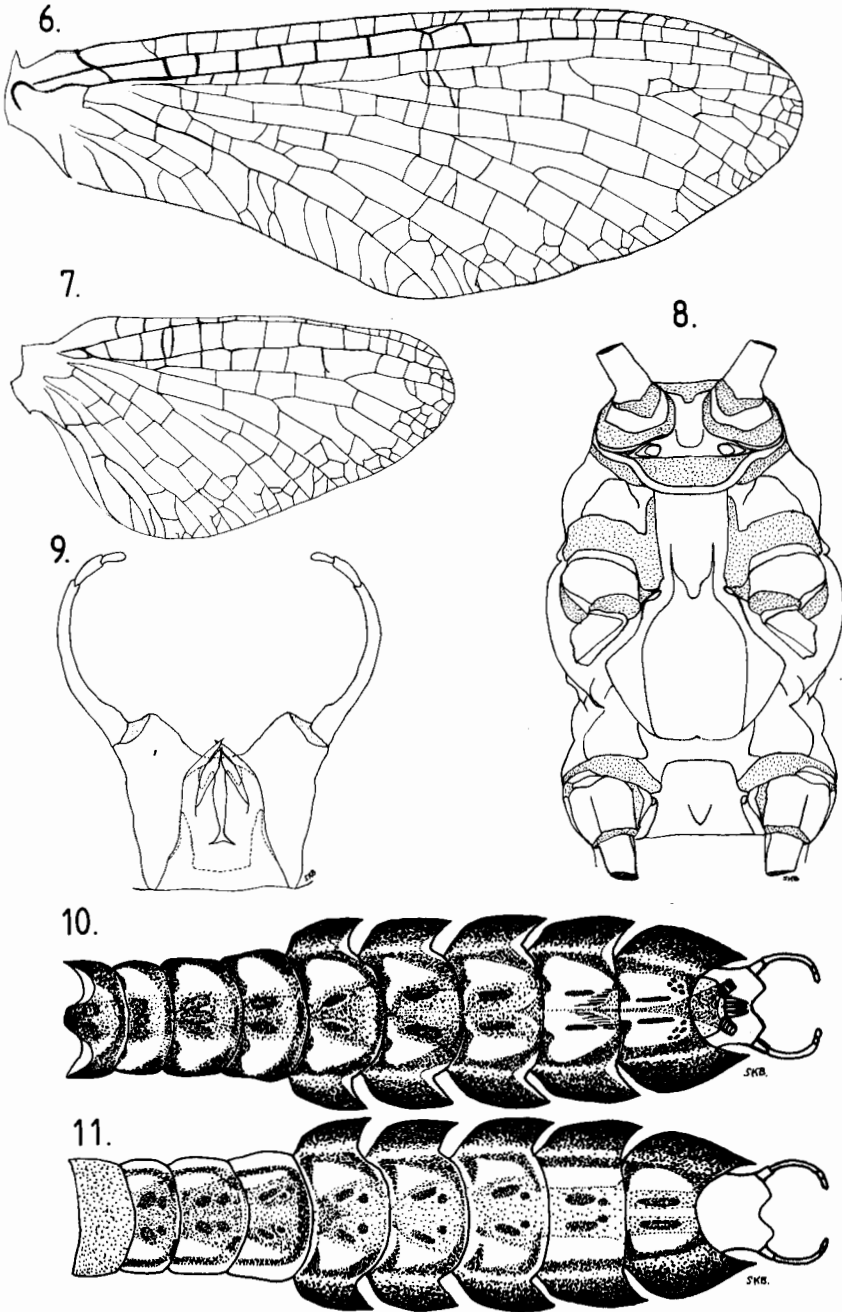
Figs. 6-11. Male imago of Siphlonisca aerodromia : 6 - forewing; 7 - hindwing; 8 - ventral view of thoracic sternae; 9 - dorsal view of genitalia; 10 - dorsal view of abdomen; 11 - ventral view of abdomen.
