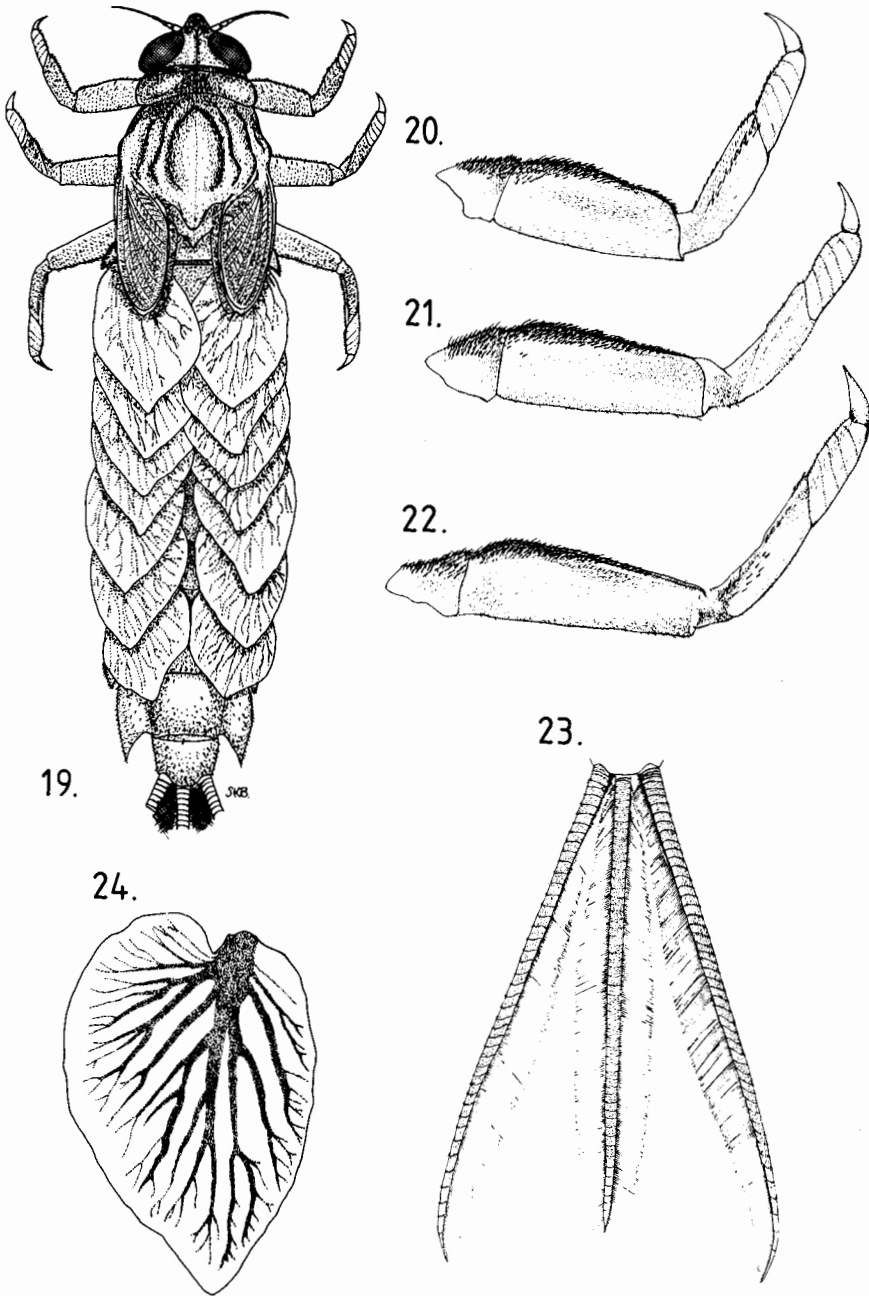
Figs. 19-24. Mature nymph of Siphlonisca aerodromia : 19 - mature nymph dorsal view; 20 - prothoracic leg; 21 - mesothoracic leg; 22 - metathoracic leg; 23 - dorsal view of caudal filaments; 24 - subcordate gill from abdominal segment 3.
