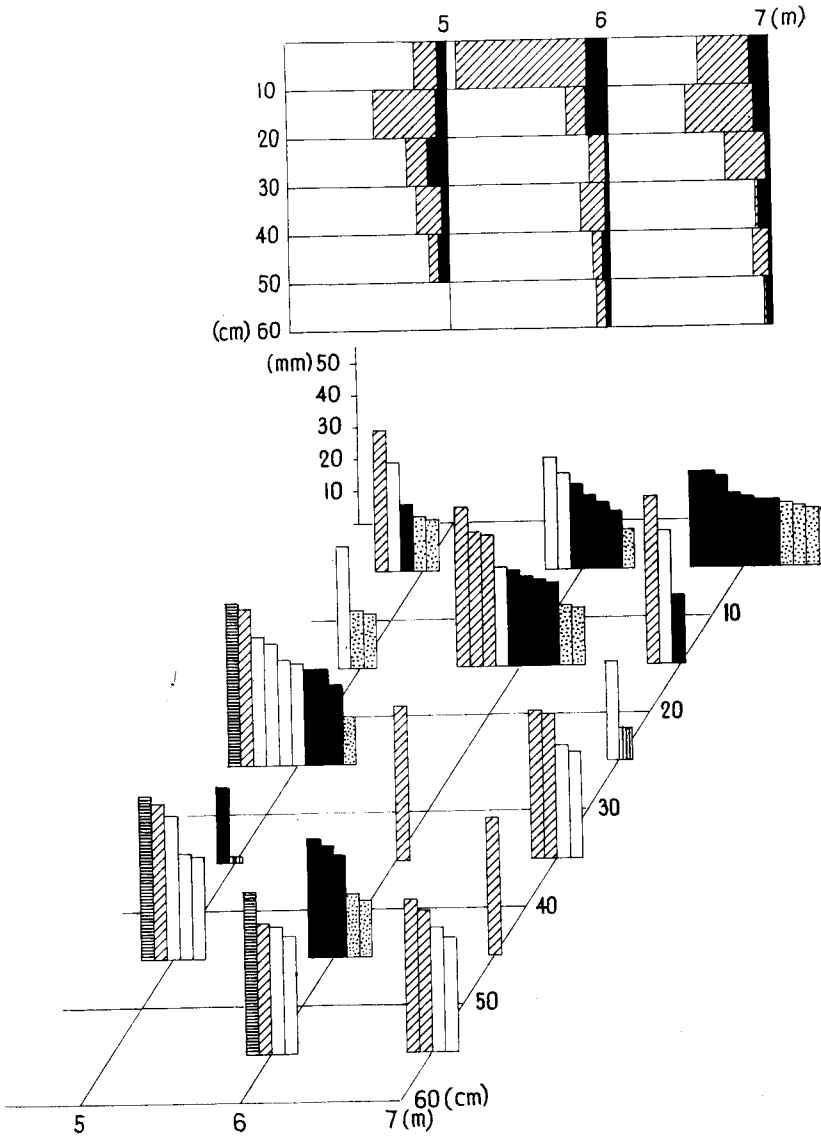
Graph 1, b: Horizontal and vertical distributions of mayfly larvae of different sizes.
