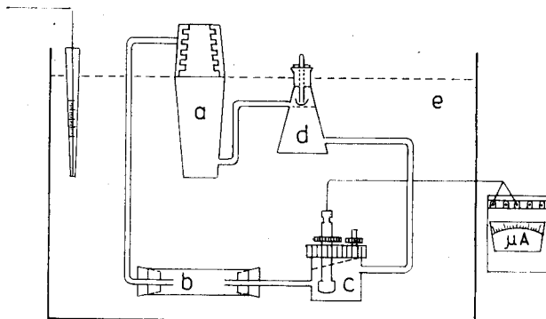
Fig. 1. Schematical representation of the apparatus measuring the flowing-water oxygen consumption. (a: water-circulator, b: respirotory chamber, c: measuring chamber, d: carbon dioxide adsorber, e: water bath).
