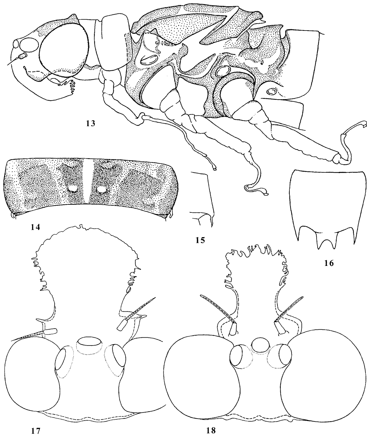
Figs 13–18. Oligoncuria itayana sp.n., adults: 13 — head and thorax of female imago (cuticular pigmentation is shown by dots; hypodermal pigmentation, which is much darker and masks it, is not shown); 14 — spread 5 th abdominal tergite of female imago (hypodermal pigmentation is shown by dots); 15 — posterolateral spine of 5 th abdominal segment of male imago (holotype); 16 — ventral side of 9 th abdominal segment of female imago; 17 — head of female subimago just after hatching from larva (imaginal cuticle is shown by interrupted line); 18 — the same, male (holotype).
