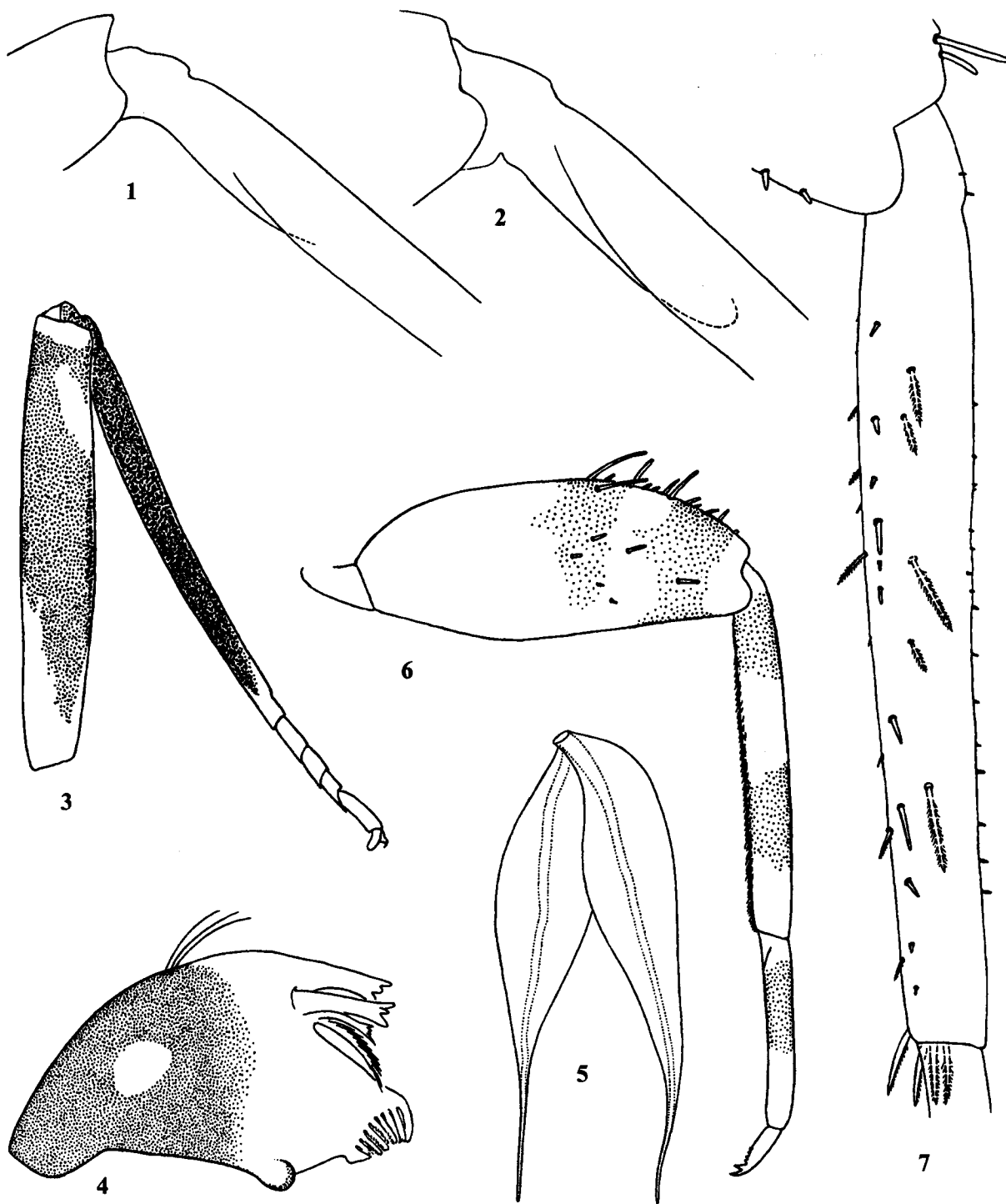
Figs 1-7: 1-2 — Meridialaris tintinnabula : 1 — proximal part of hind tibia, subimago; 2 — the same, larva; 3-7 — Simothraulopsis (Maculognathus) sabalo sp.n. (3, 4, 6, 7 — holotype): 3 — hind leg of imago; 4-7 — larva: 4 — left mandible; 5 — right tergite III; 6 — fore leg (cuticular pigmentation shown by dots, hypodermal pigmentation not shown; long fine setae on outer margin of femur, tibia and tarsus not shown); 7 — tibia of hind leg (bipectinate setae on opposite side shown by interrupted line; long fine setae on outer margin not shown).
