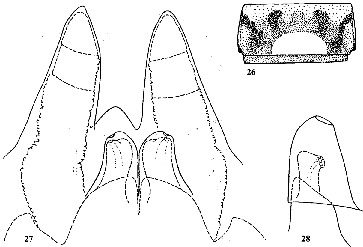
Figs 26–28. Farodes spp.: 26 — F. pakitza , abdominal tergite VII of male imago, spread on slide; 27–28 — F. bimaculatus from Cuba: 27 — genitalia of mature male larva ready to moult to subimago, dorsal view (buds of subimaginal penis and gonostyli shown by interrupted line); 28 — a half of larval protopenis with bud of subimaginal penis just before moult to subimago, dorsal-medial view.
