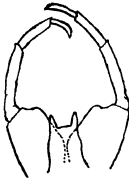
FIG. 47.— Coloburiscus humeralis. Genitalia of male imago. \times 25 .
