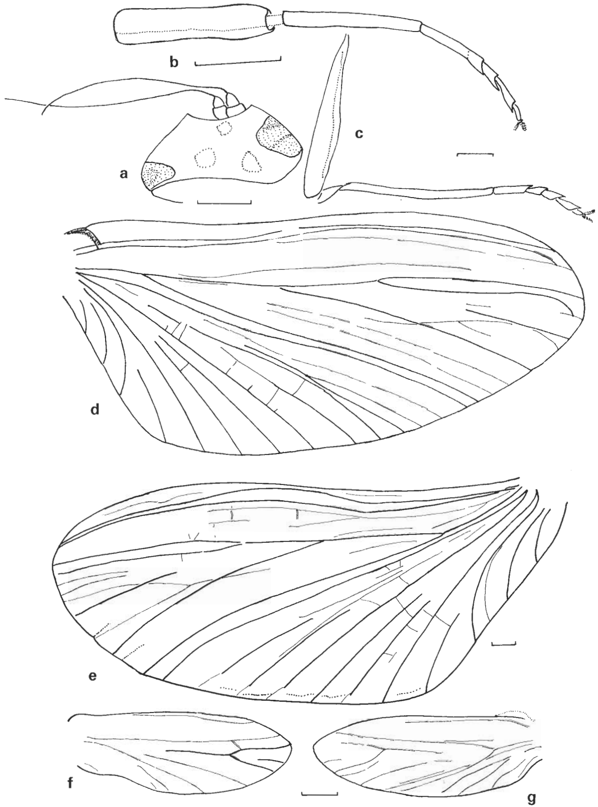
Fig. 1 Myanmarrella rossi gen. nov. sp. nov., holotype. In.20173. Burmese amber. a , head, scale 0.01 mm; b , fore leg; c , middle leg; d , right fore wing; e , left fore wing; f , right hind wing; g , left hind wing; scales for b – g 0.1 mm.
