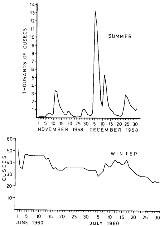
Fig. 3. Daily variation in the flow of the Vaal River at Standerton in the Summer (wet season) and in the Winter (dry season). (1 cusec equals 28.32 litres per second).
