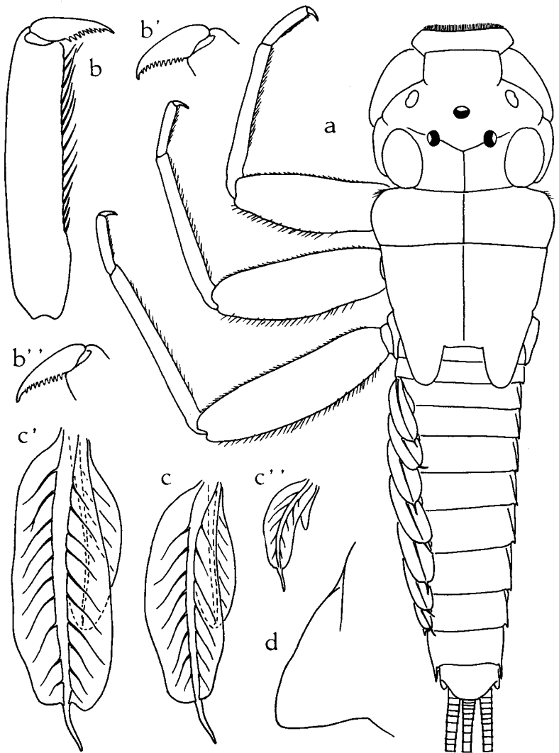
Fig. 1. — Atalophlebioides inequalis sp. nov., larve holotype.
