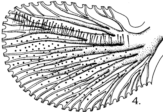
FIG. 4.—Lower surface of the 1st oscillating gill. Campaniform sensillae are shown posterior to the band of trichoid sensillae.
