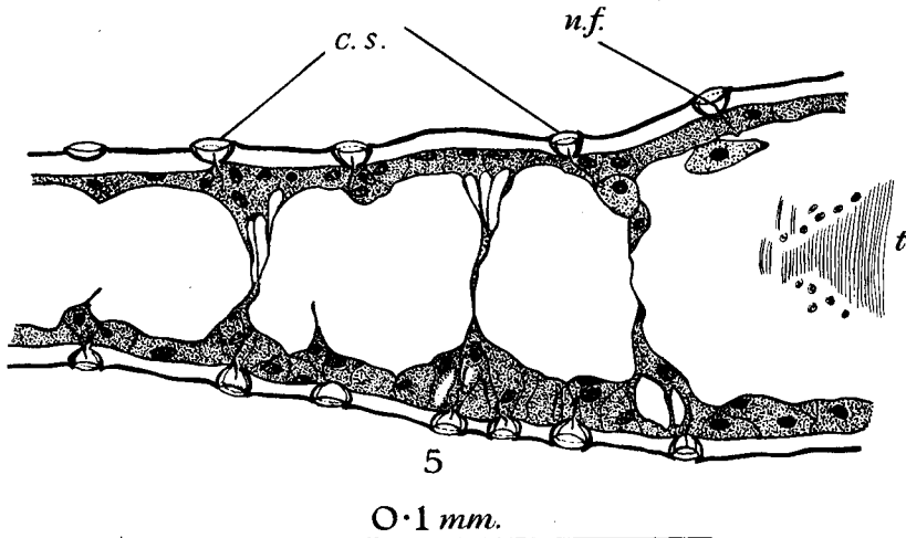
FIG. 5.—Transverse section across a gill. c.s. , campaniform sensillae; n.f. , nerve fibril; t. , trachea.
