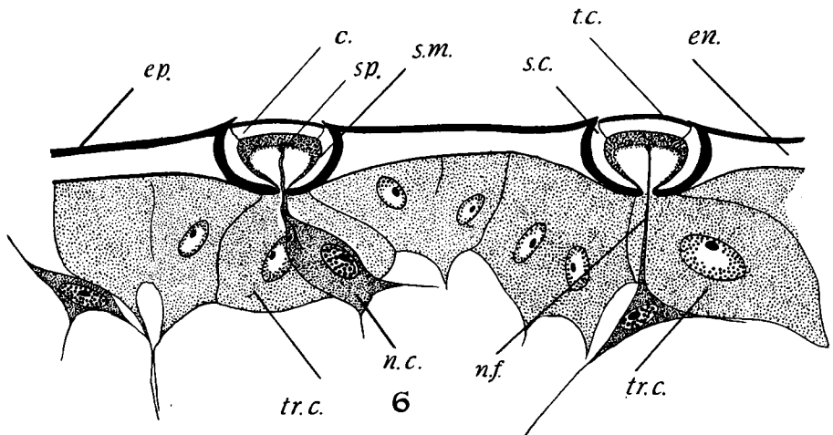
FIG. 6.—Composite diagram of a vertical section through two campaniform sensillae. c. , cushion to the terminal cap; en. , endocuticle; ep. , epicuticle; n.c. , nerve cell; n.f. , nerve fibril; s.c. , sensillary cup; s.m. , supporting membrane; sp. , scolopale; t.c. , terminal cap; tr.c. , trichogen cell.
