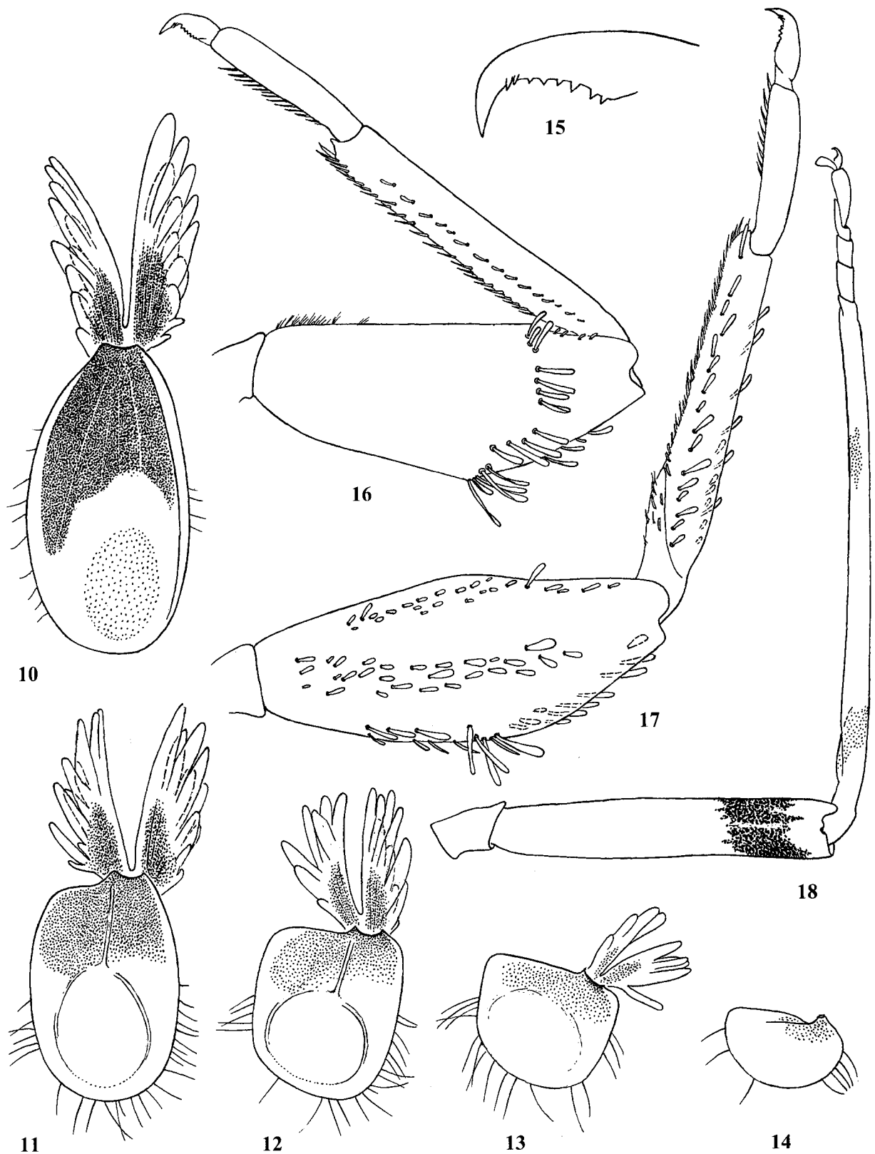
Figs 10-18. Ephemerythus niger ugandanus subsp.n.: 10-17 — larva: 10-14 — tergitei II-VI with ventral portions turned out; 15 — claw; 16-17 — fore and middle legs, dorsal view; 18 — middle leg of male imago.
