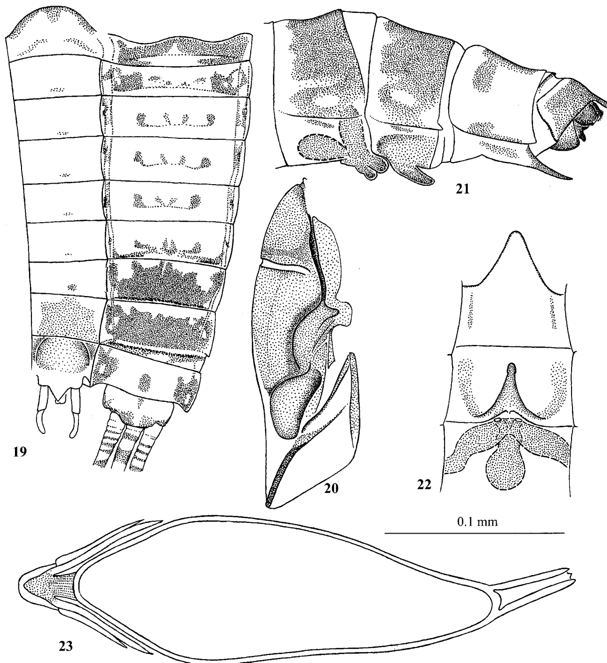
Figs 19–23. Ephemerythus niger ugandanus subsp.n.: 19 — abdomen of male imago, spread on slide (hypodermal pigmentation shown by dots); 20 — subimaginal exuviae of right half of mesonotum (cuticular pigmentation shown by dots); 21 — abdominal segments VII–X of female imago, lateral view (hypodermal pigmentation shown by dots, internal genitalia shown by interrupted line); 22 — the same, ventral view; 23 — optic section of egg with scale bar; 19–20 — holotype.
