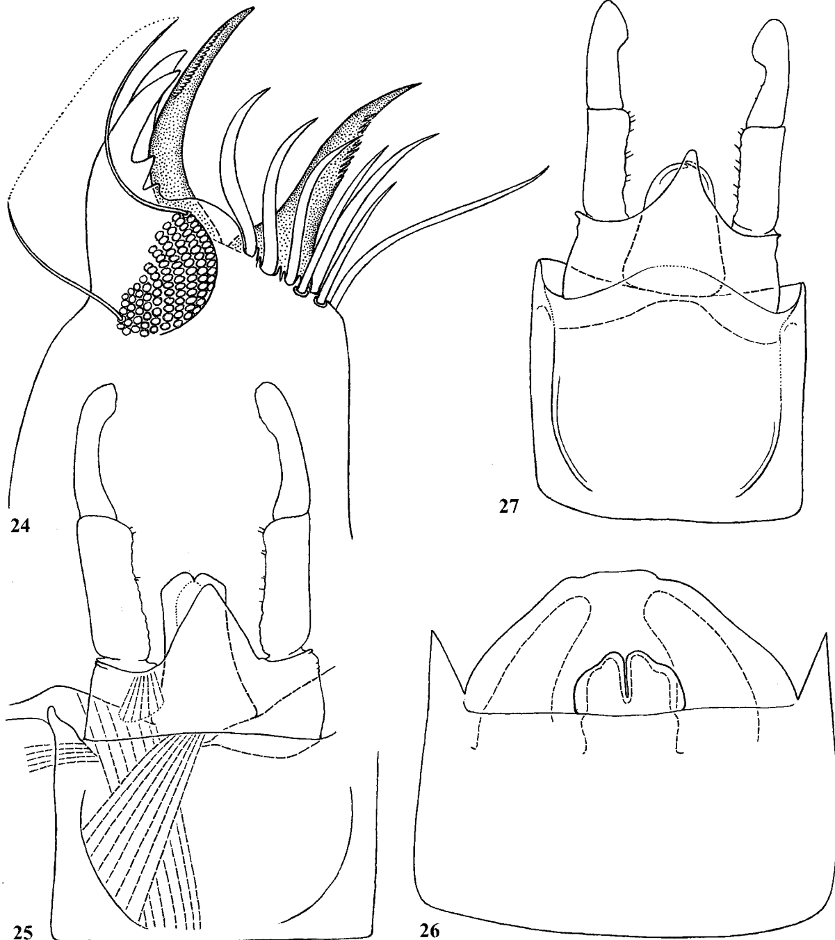
Figs 24–27. 24–26 — Ephemerythus niger ugandanus subsp.n., 27 — E. kiboensis ; 24 — apex of maxilla, ventral view (dentisetae shown by dots; most part of apical setae not shown, area occupied by them shown by dotted line); 25 — genitals of male imago, holotype, ventral view (musculature of left half shown by interrupted lines); 26 — abdominal sternum XI of male larva, dorsal view (hypodermal rudiments of future subimaginal penis and gonostyli shown by interrupted lines). 27 — genitals of male imago, ventral view.
