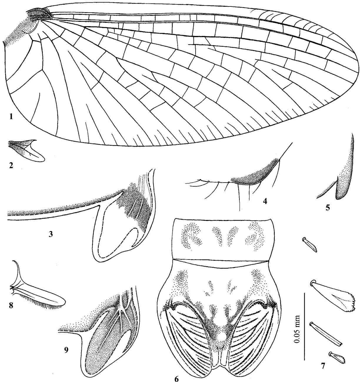
Figs 1–9. 1–7 — Ephemerythus niger ugandanus subsp.n.; 8–9 — Leptohiphes zalope ; 1–2 — fore and hind wings of male imago at the same scale; 3 — hind protopteron of last instar male larva, with hypoderm shown by interrupted line; 4 — hind protopteron of last instar female larva; 5 — hind wing of female imago (Figs 3–5 at the same scale); 6 — larval pronotum and mesonotum (outlines of hypodermal rudiments of wings and plumidia shown by interrupted line; hypodermal pigmentation shown by dots; cuticular pigmentation not shown); 7 — setae on mesonotum with scale bar; 8 — hind wing of male imago; 9 — hind protopteron of last instar male larva, with hypoderm shown by interrupted line [8 and 9 from Kluge, 2004].
