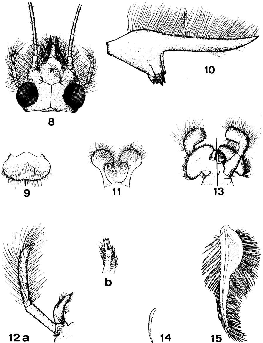
FIGS. 8-15. Litobrancha recurvata , nymph. 8. Head, dorsal view. 9. Labrum, anterior view. 10. Right mandibular tusk, lateral view. 11. Hypopharynx. 12a. Right maxilla posterior view. 12b. Galea-lacinia, median view. 13. Labium. 14. Abdominal gill 1. 15. Dorsal section of right gill 2.
