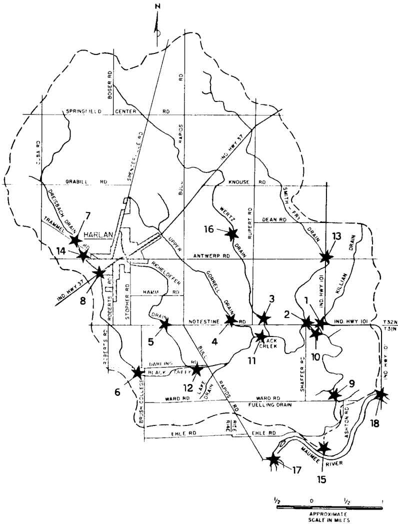
Fig. 1. Sampling sites of the Black Creek drainage area and Maumee River.
