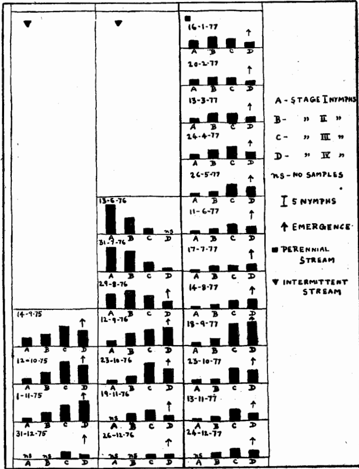
Gen. et. sp. nov. A Fig. 2. Petersula courtallensis —age frequency histograms
